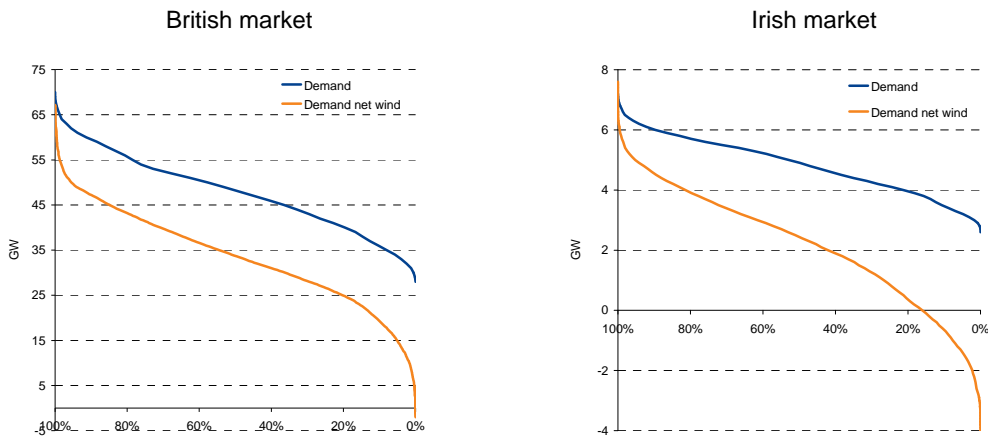
Figure 6 – Demand duration curves for both markets in 2030
